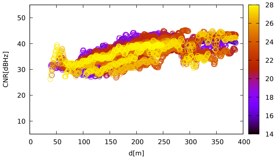
CNR vs distance (LeicaGS18 for G26 at L1)
