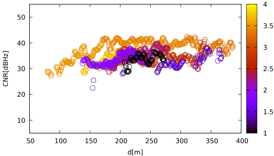
CNR vs distance (LeicaGS18 for G32 at L1)
