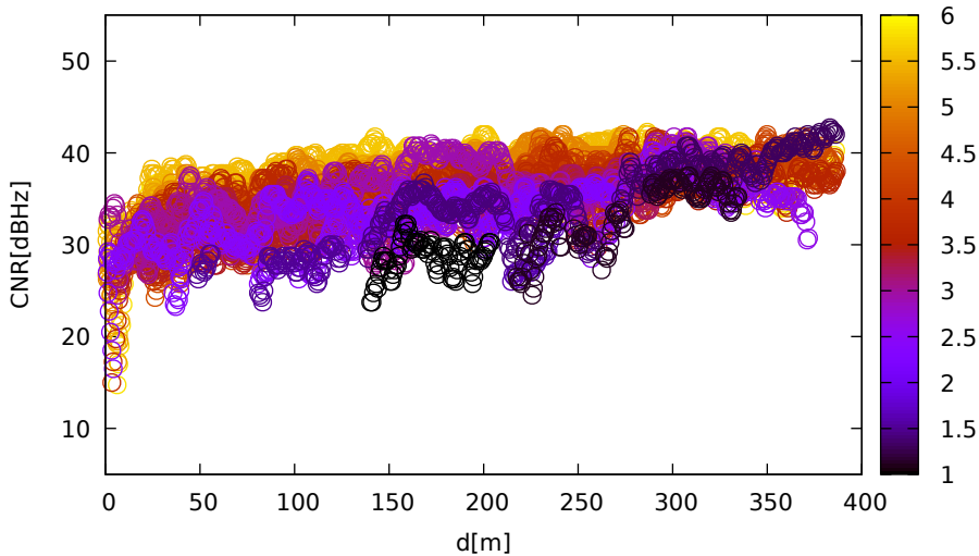
CNR vs distance (LeicaGS18 for R03 at L1)
