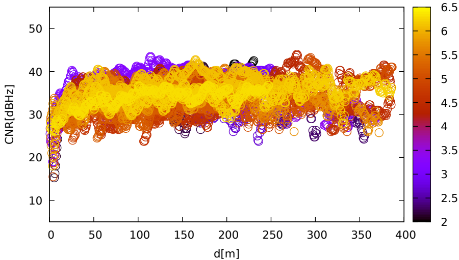
CNR vs distance (LeicaGS18 for R04 at L1)
