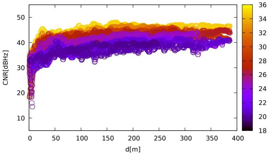
CNR vs distance (LeicaGS18 for R10 at L1)
