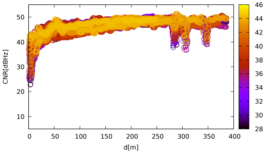
CNR vs distance (LeicaGS18 for R12 at L1)
