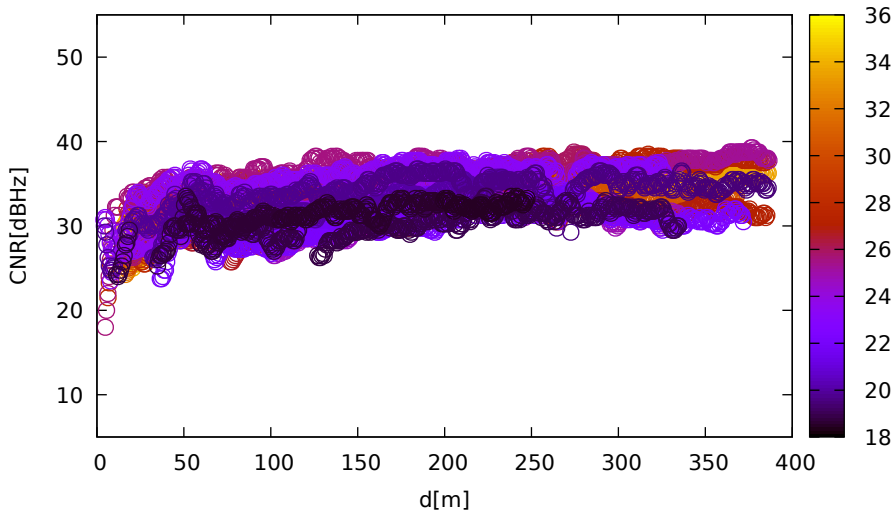
CNR vs distance (LeicaGS18 for R20 at L1)
