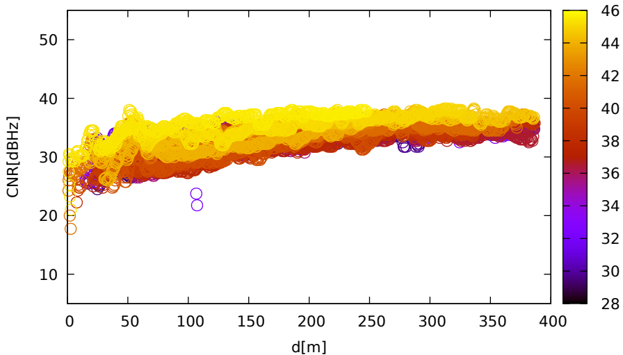
CNR vs distance (LeicaGS18 for R22 at L1)
