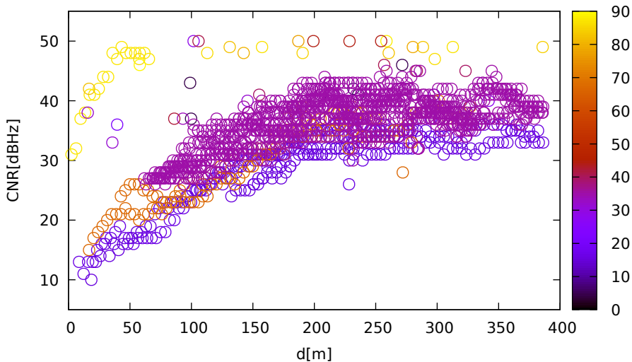
CNR vs distance (UbloxF9R for 123 at L1)
