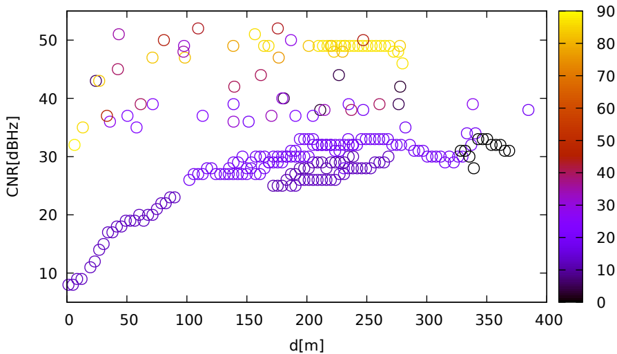
CNR vs distance (UbloxF9R for 126 at L1)
