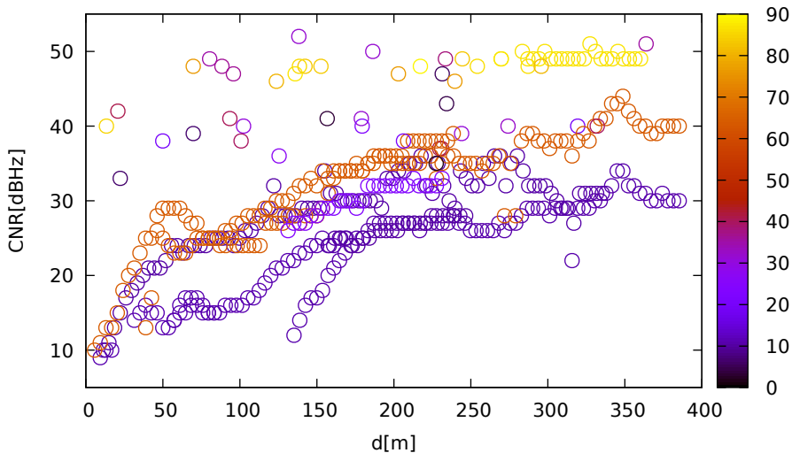
CNR vs distance (UbloxF9R for 127 at L1)
