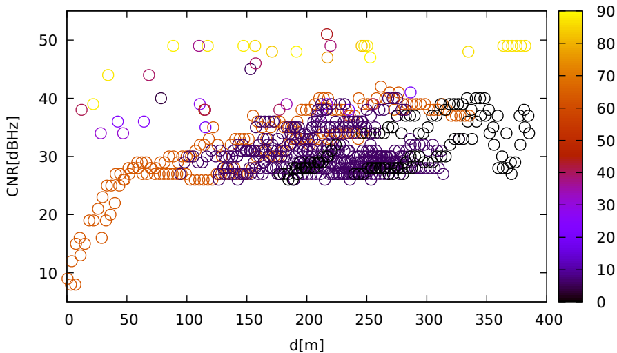
CNR vs distance (UbloxF9R for 128 at L1)
