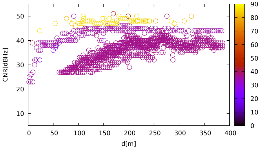
CNR vs distance (UbloxF9R for 136 at L1)
