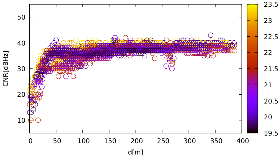
CNR vs distance (UbloxF9R for C08 at L1)
