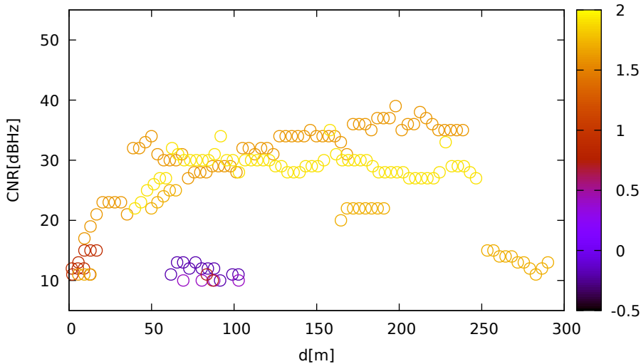
CNR vs distance (UbloxF9R for C14 at L1)
