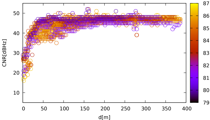
CNR vs distance (UbloxF9R for C27 at L1)
