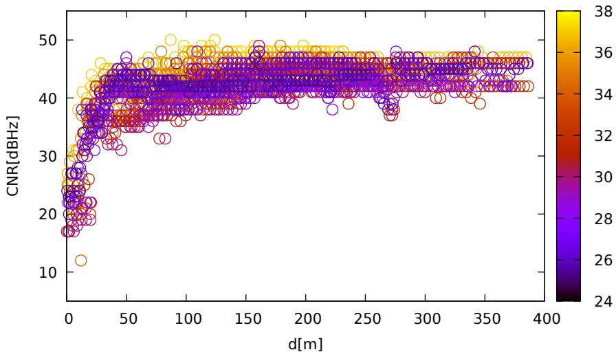
CNR vs distance (UbloxF9R for C28 at L1)
