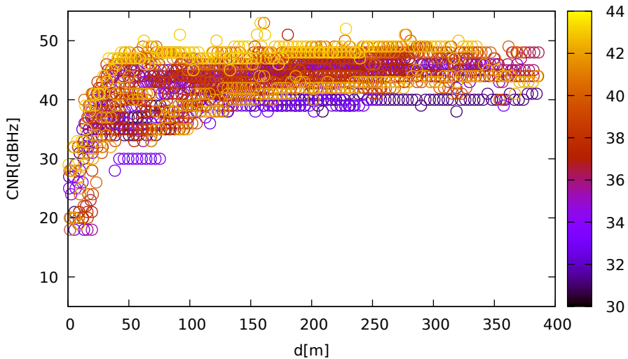
CNR vs distance (UbloxF9R for C30 at L1)
