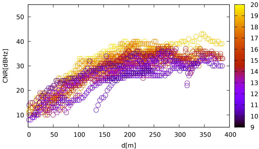
CNR vs distance (UbloxF9R for E01 at L1)
