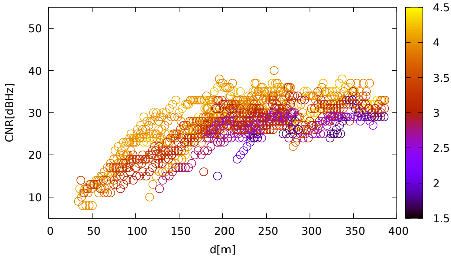
CNR vs distance (UbloxF9R for E03 at L1)
