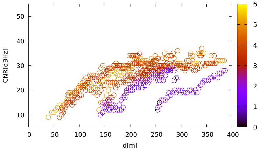
CNR vs distance (UbloxF9R for E05 at L1)
