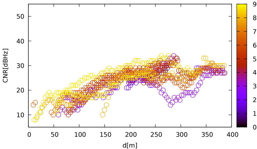
CNR vs distance (UbloxF9R for E11 at L1)
