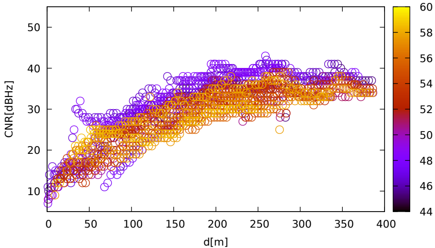
CNR vs distance (UbloxF9R for E12 at L1)
