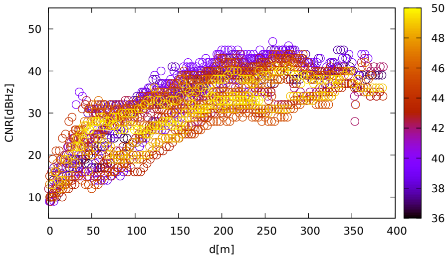
CNR vs distance (UbloxF9R for E14 at L1)
