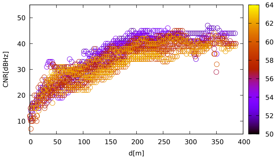
CNR vs distance (UbloxF9R for E24 at L1)
