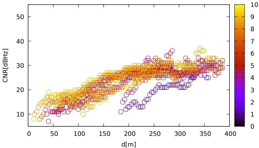
CNR vs distance (UbloxF9R for E25 at L1)
