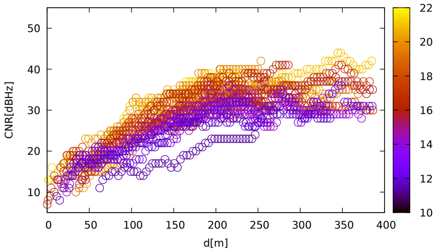
CNR vs distance (UbloxF9R for E26 at L1)
