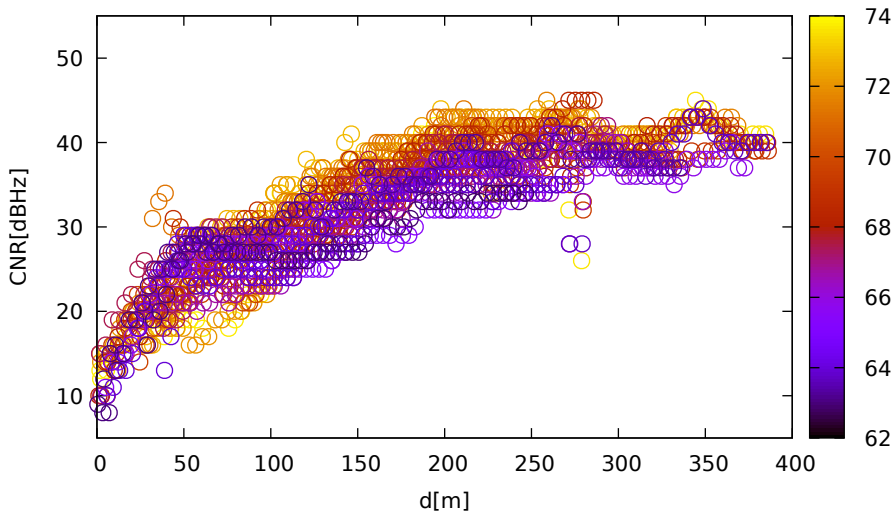
CNR vs distance (UbloxF9R for E31 at L1)
