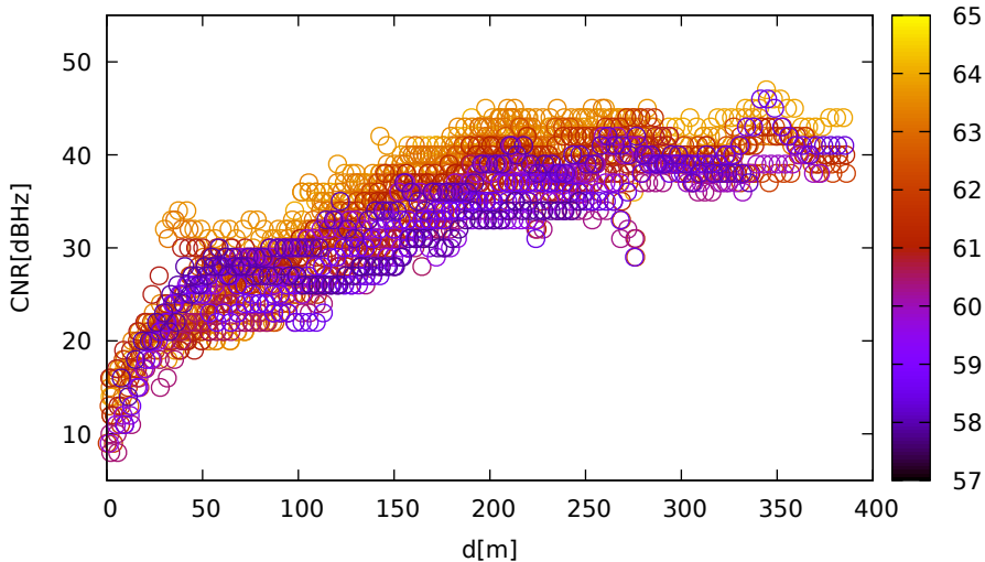
CNR vs distance (UbloxF9R for E33 at L1)
