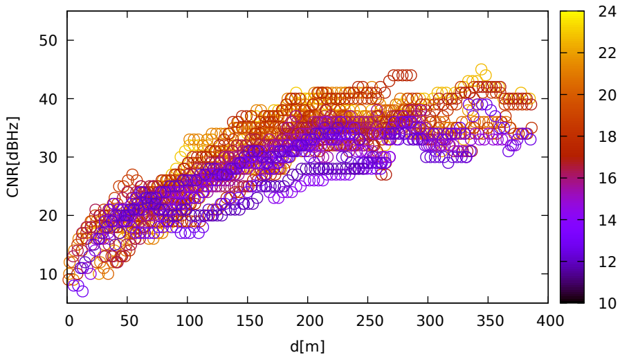
CNR vs distance (UbloxF9R for G02 at L1)
