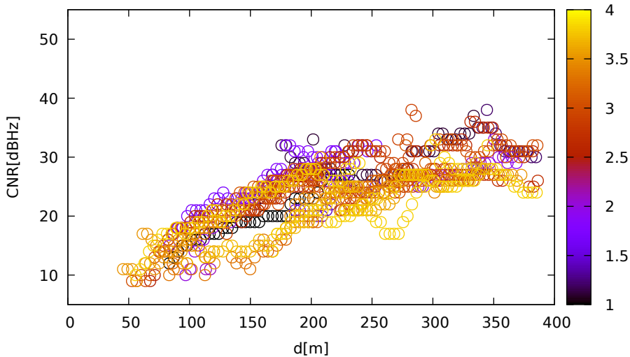
CNR vs distance (UbloxF9R for G04 at L1)
