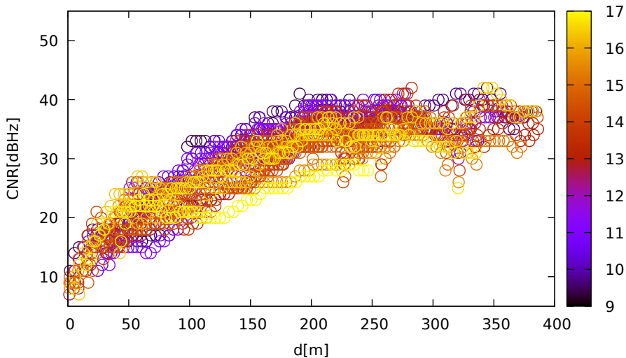
CNR vs distance (UbloxF9R for G05 at L1)
