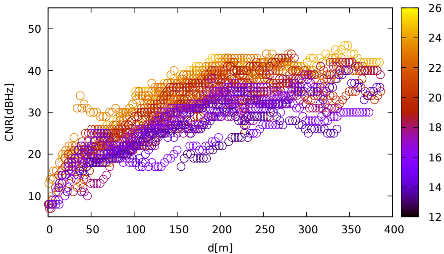
CNR vs distance (UbloxF9R for G12 at L1)
