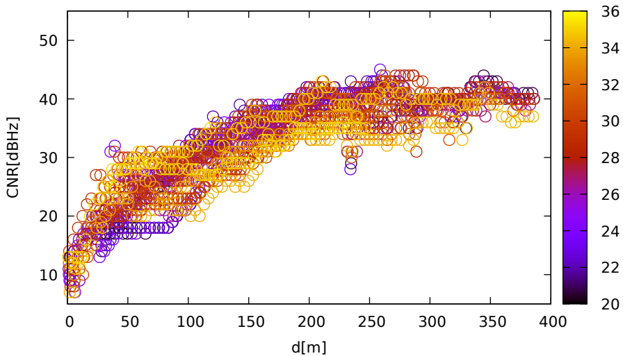
CNR vs distance (UbloxF9R for G18 at L1)
