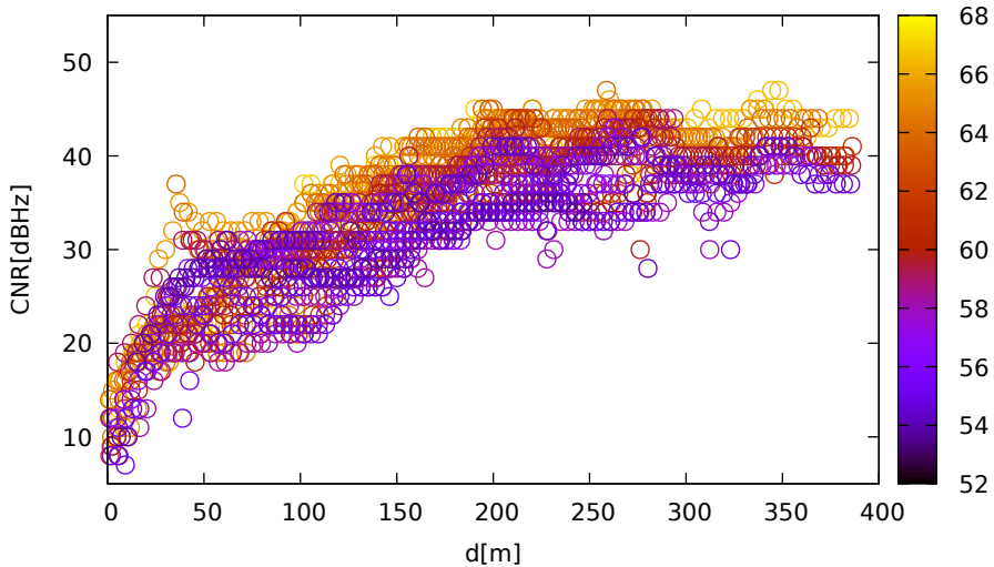
CNR vs distance (UbloxF9R for G25 at L1)
