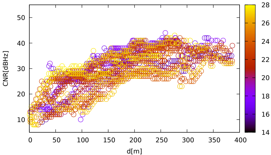
CNR vs distance (UbloxF9R for G26 at L1)
