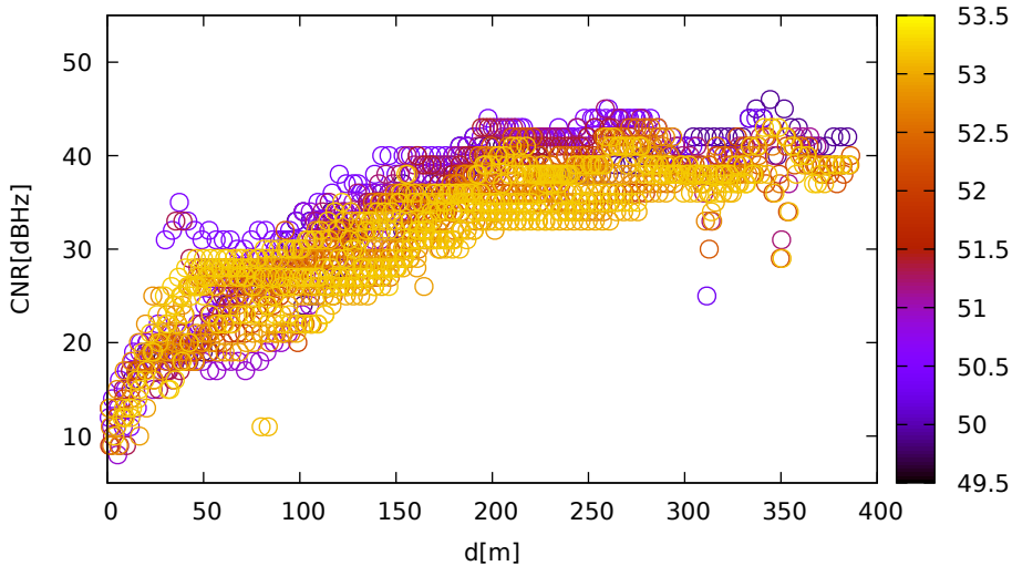
CNR vs distance (UbloxF9R for G31 at L1)
