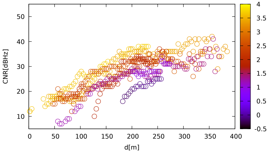
CNR vs distance (UbloxF9R for G32 at L1)
