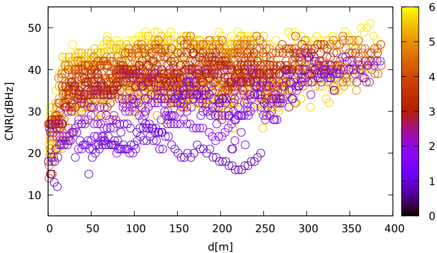
CNR vs distance (UbloxF9R for R03 at L1)
