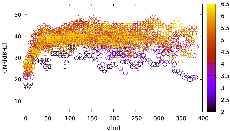
CNR vs distance (UbloxF9R for R04 at L1)
