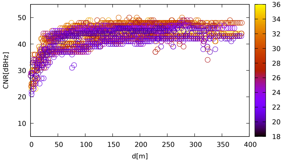
CNR vs distance (UbloxF9R for R10 at L1)
