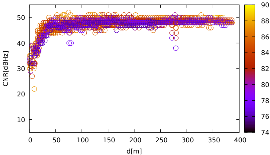
CNR vs distance (UbloxF9R for R11 at L1)
