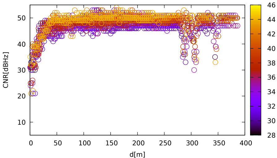
CNR vs distance (UbloxF9R for R12 at L1)
