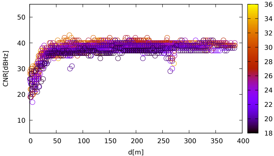
CNR vs distance (UbloxF9R for R20 at L1)
