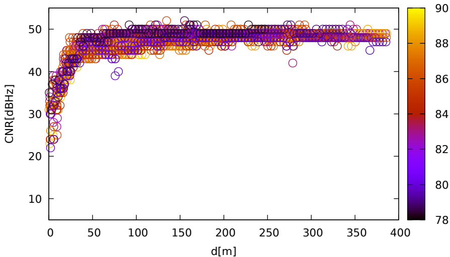
CNR vs distance (UbloxF9R for R21 at L1)
