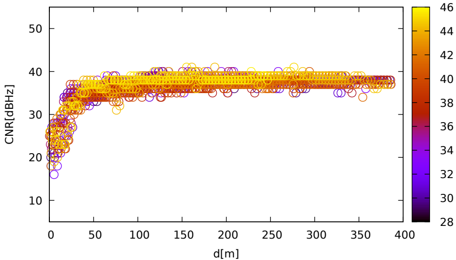
CNR vs distance (UbloxF9R for R22 at L1)
