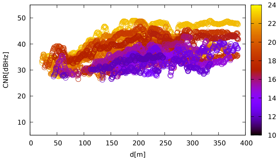
CNR vs distance (LeicaGS18 for G02 at L1)
