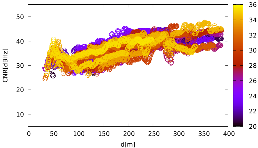
CNR vs distance (LeicaGS18 for G18 at L1)
