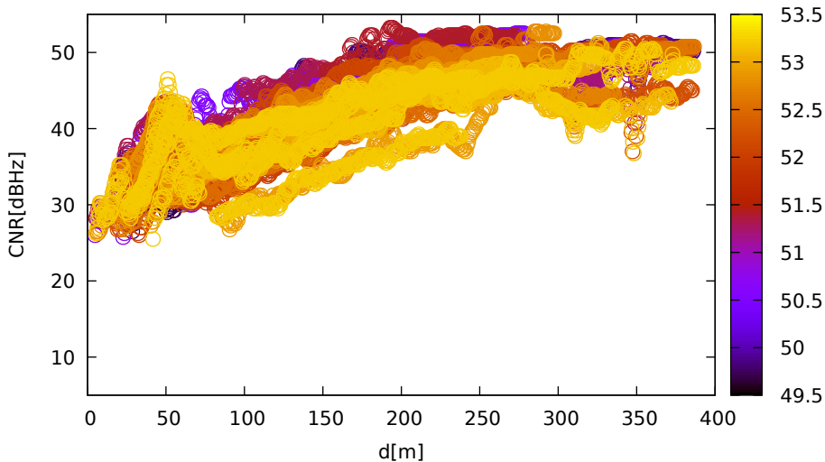
CNR vs distance (LeicaGS18 for G31 at L1)
