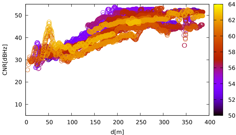
CNR vs distance (LeicaGS18 for E24 at L1)
